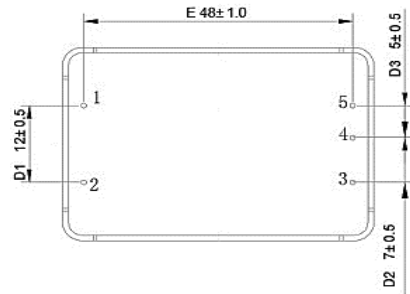
ZP series 10W dual output
