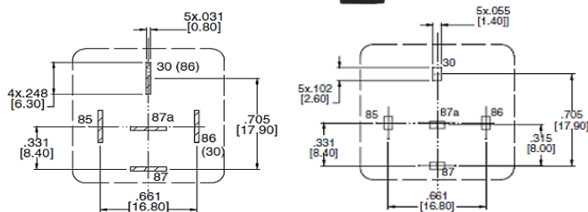
Socket: ST9721 series
